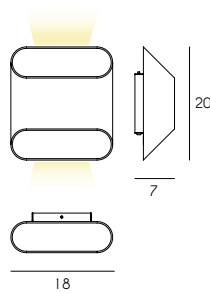
1M1240 S P LED 4,5+4,5W
