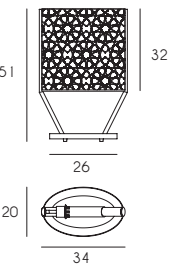
1M1279 E27 LED max 10W
