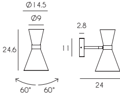
1M1293 FV E27 LED MAX 8W
