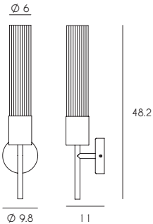
1M1272 FV E27 LED MAX 8W
