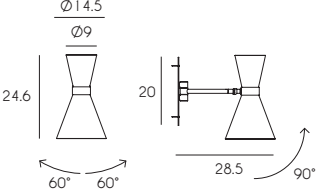
1M1285 FV E27 LED max 8W
