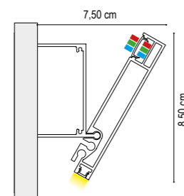
FLOAT K LED MONOCOLORE + RGB
