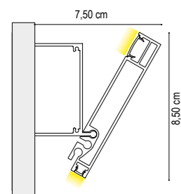
FLOAT K LED MONOCOLORE
