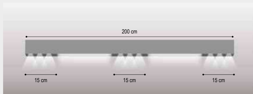
VISTA FRONTALE / FRONT VIEW
