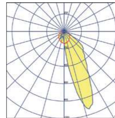
LENTE WALL WASHER - 45° WALL WASHER LENS - 45°
