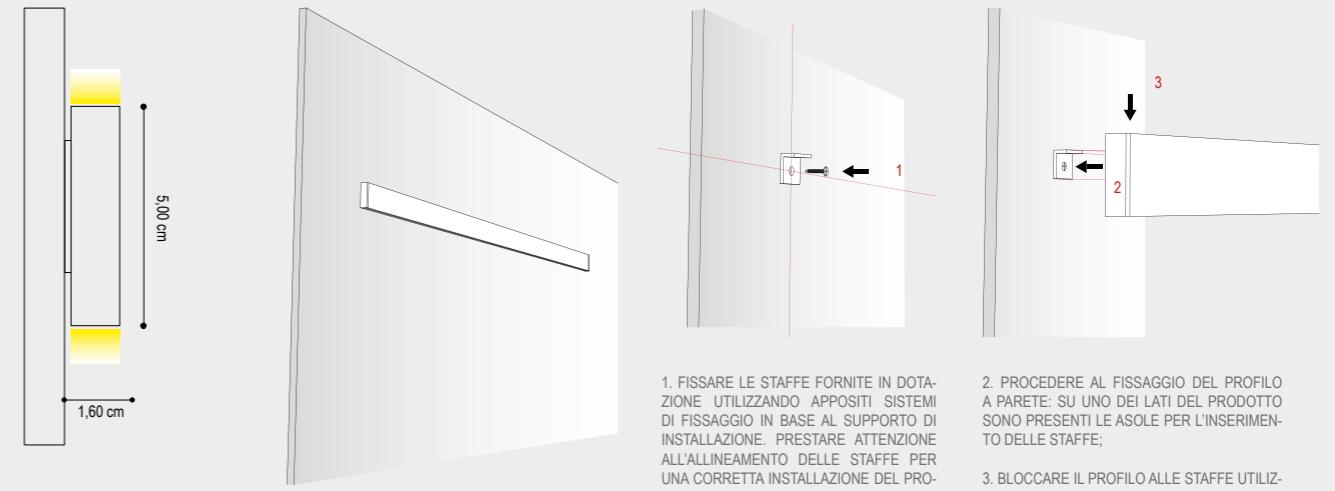
DAVINCI CON DRIVER REMOTO DAVINCI WITH REMOTE DRIVER
