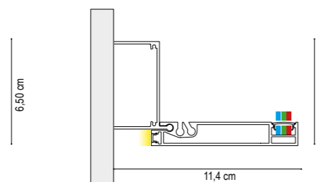
FLOAT L LED MONOCOLORE + RGB
