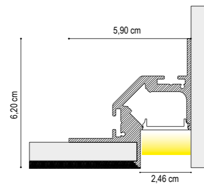
KEPLER CON COVER ESTERNA KEPLER WITH EXTERNAL COVER
