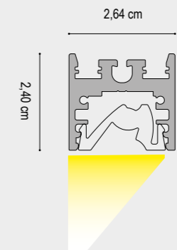
VERSIONE WALL WASHER (45°) WALL WASHER VERSION (45°)
