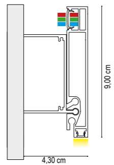
FLOAT I LED MONOCOLORE + RGB
