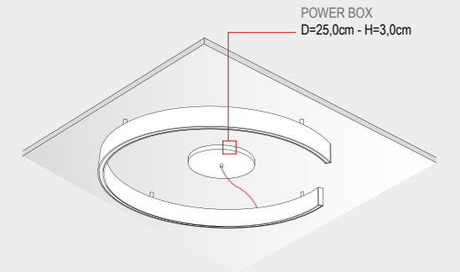
ALTIS CON BOX ALTIS WITH POWER SUPPLY BOX
