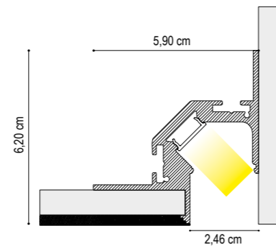
KEPLER CON COVER RECESSA KEPLER WITH RECESSED COVER
