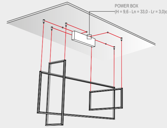
XYZ CON BOX XYZ WITH POWER SUPPLY BOX
