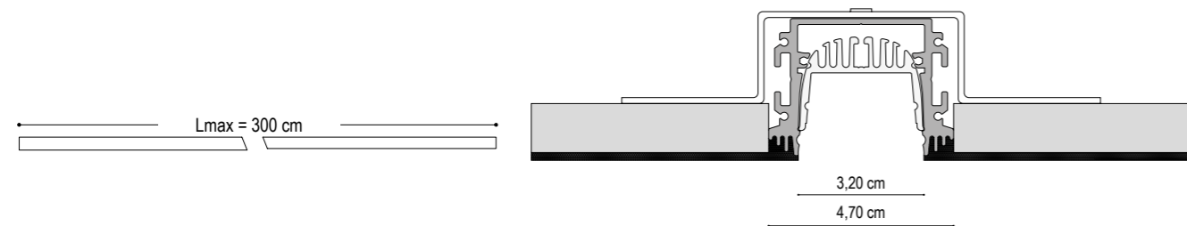
Profilo in alluminio Profile in aluminum
