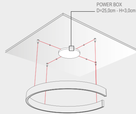
ALTIS CON BOX ALTIS WITH POWER SUPPLY BOX
