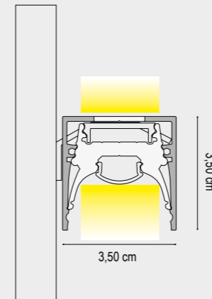
ZER035X-P CON DIFFUSORE RECESSO ZER035X-P WITH RECESSED DIFFUSER
