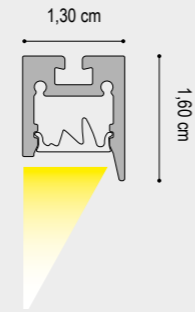
VERSIONE WALL WASHER (45°) WALL WASHER VERSION (45°)
