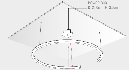
KRONOS CON BOX KRONOS WITH POWER SUPPLY BOX
