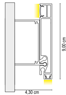
FLOAT I LED MONOCOLORE
